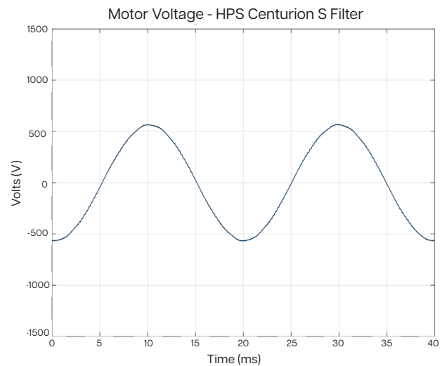
Motor Voltage With HPS Centurion S Filter
