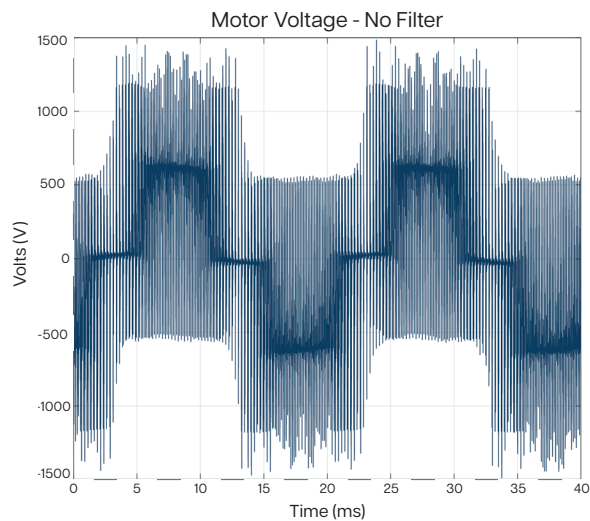
Motor Voltage No Filter
