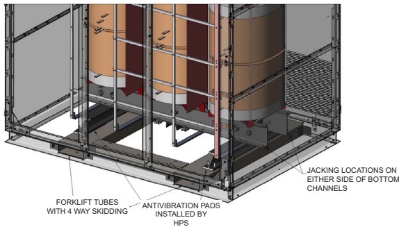
FIGURE 11: OPTIONAL FORKLIFT BASE WITH 4 WAY SKIDDING
